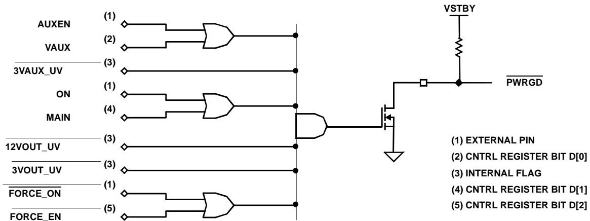
FIGURE 30. \overline{\text{PWRGD}} LOGIC DIAGRAM
